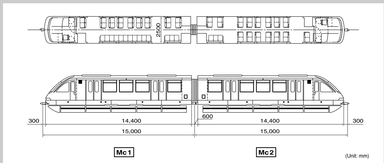
Figure 5 HSST-100L Vehicle Design
