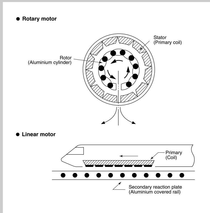
Figure 2 Principle of HSST Magnetic Propulsion
